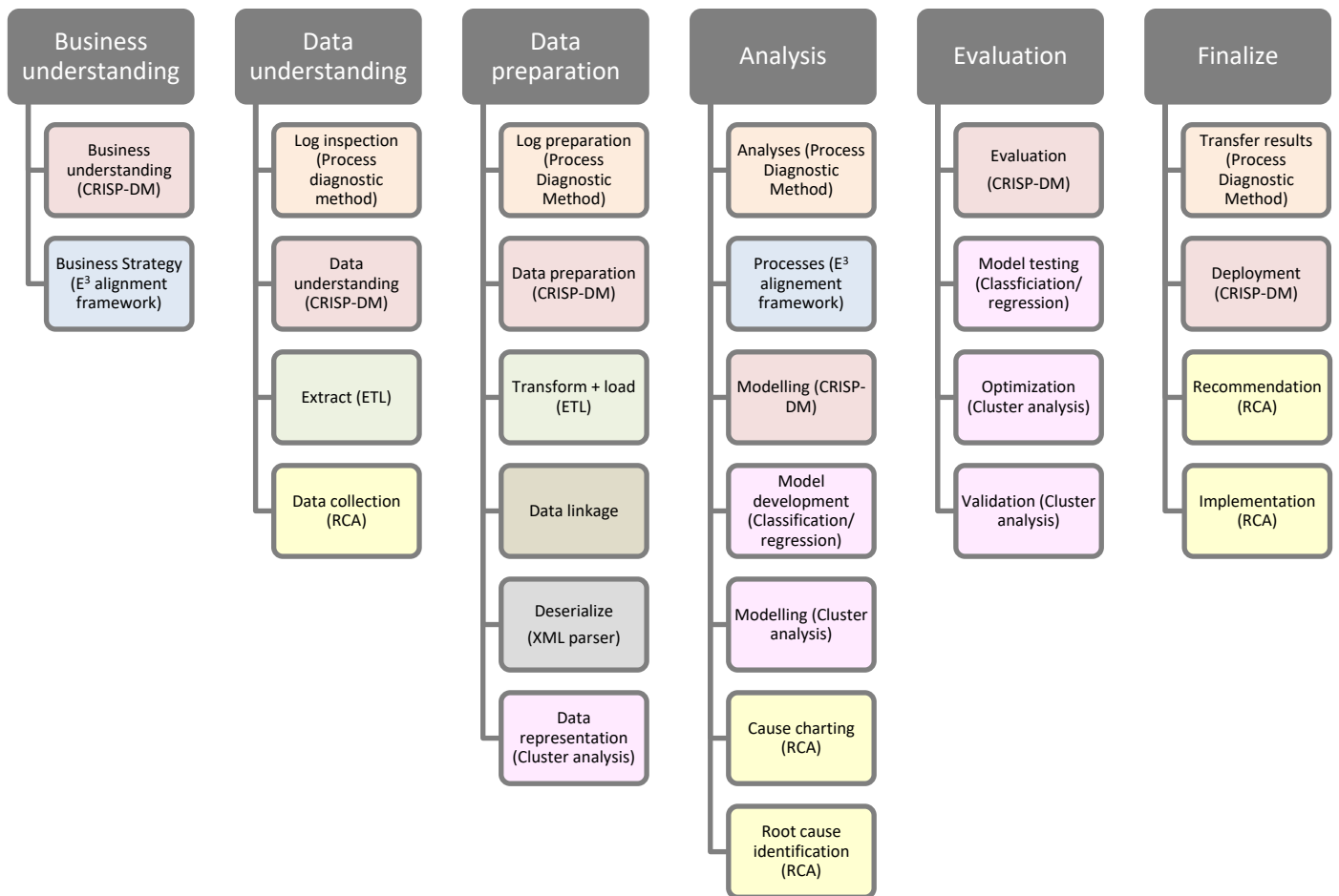
Figure 4. Framework including exploratory data analytics and RCA methods
