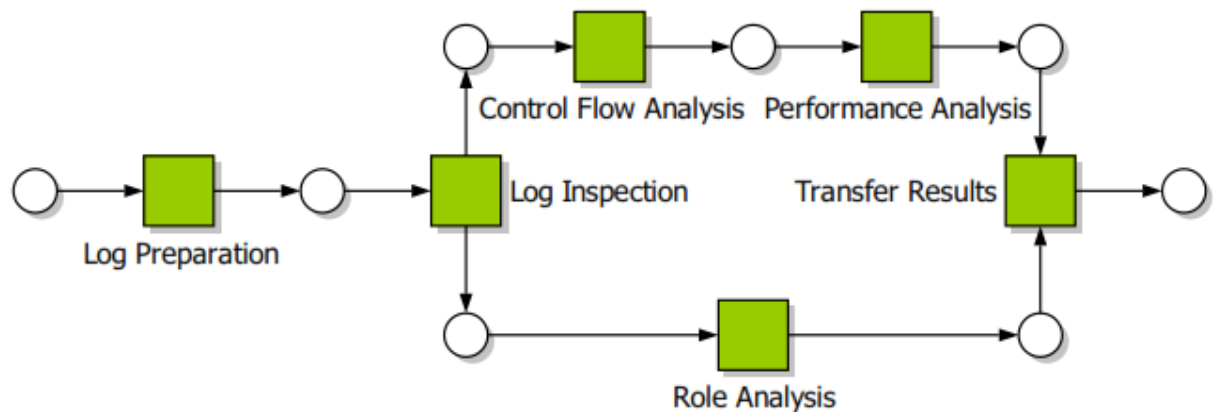
Figure 2. Process diagnostic method based on (Bozkaya et al. 2009)
